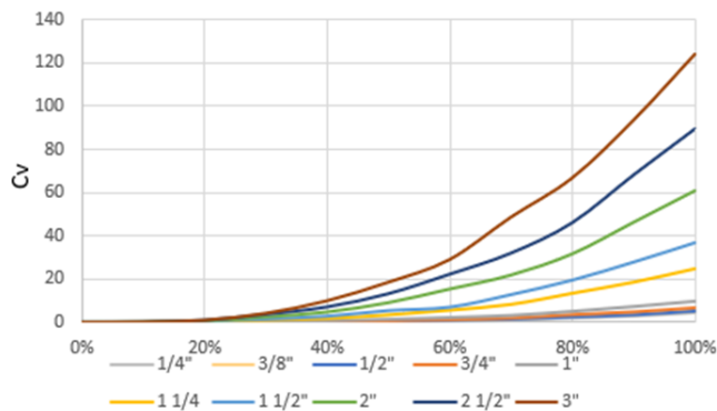
Cv vs % Open, 60° V Port
